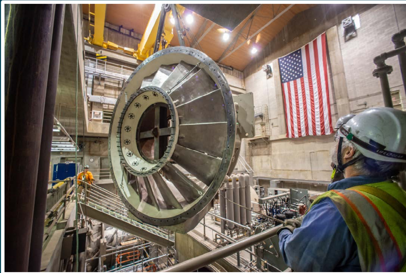
Newly refurbished 30-ton distributor with stainless steel wicket gates is lowered into Generating Unit 8
