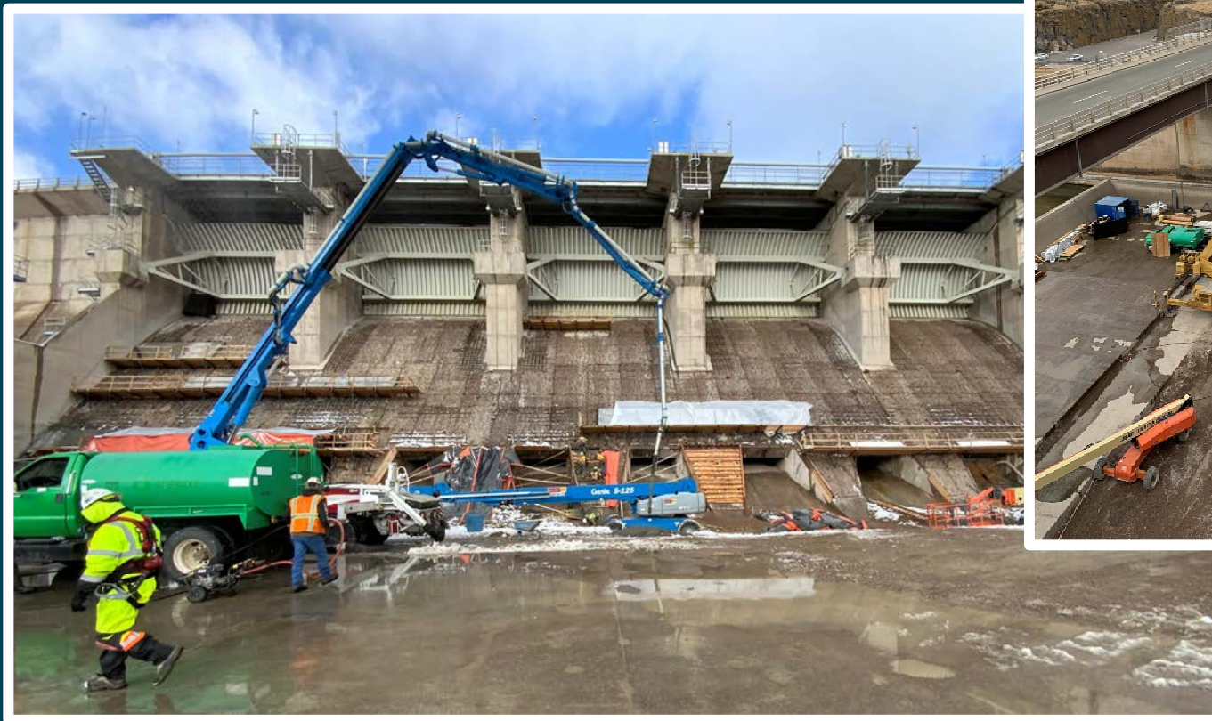
American Falls Dam downstream face spillway demolition
